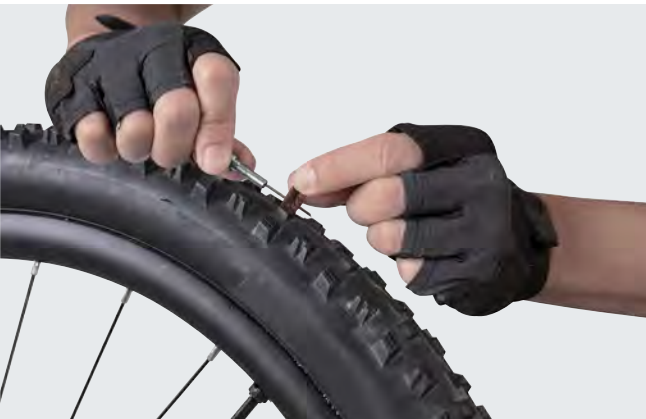
2. Remove excess plug with knife
