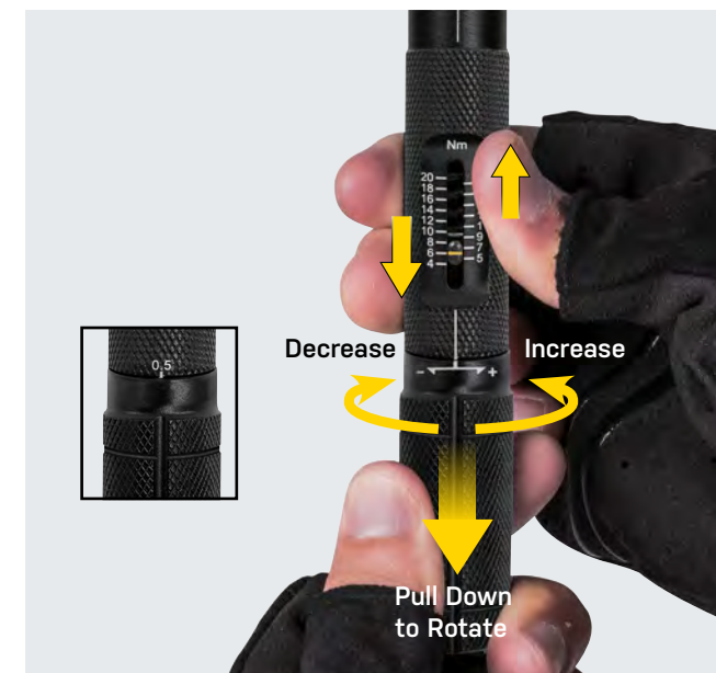
Torque wrench with adjustable preset range of 4 - 20Nm
