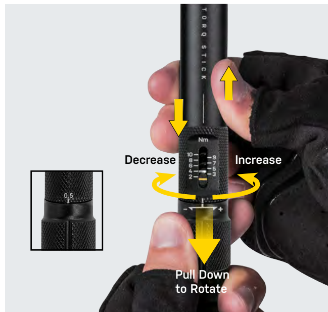
Rotate a half turn for 0.5Nm adjustment
