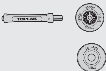
Adapter B
